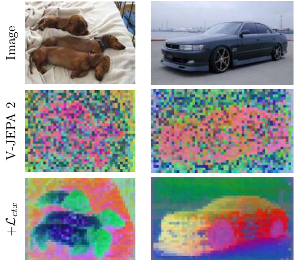
Figure 3 Influence of the context loss \mathcal{L}_{ctx} . We show PCA visualizations of the feature map representations learned with V-JEPA 2 and with a model trained using V-JEPA 2 plus our \mathcal{L}_{ctx} loss. While V-JEPA features only show fragmented local spatial structure, explicitly supervising unmasked regions with \mathcal{L}_{ctx} leads to feature maps that exhibit coherent spatial structure. Similar semantic parts (e.g., heads of dogs, wheels of cars) are mapped to the same PCA components.
